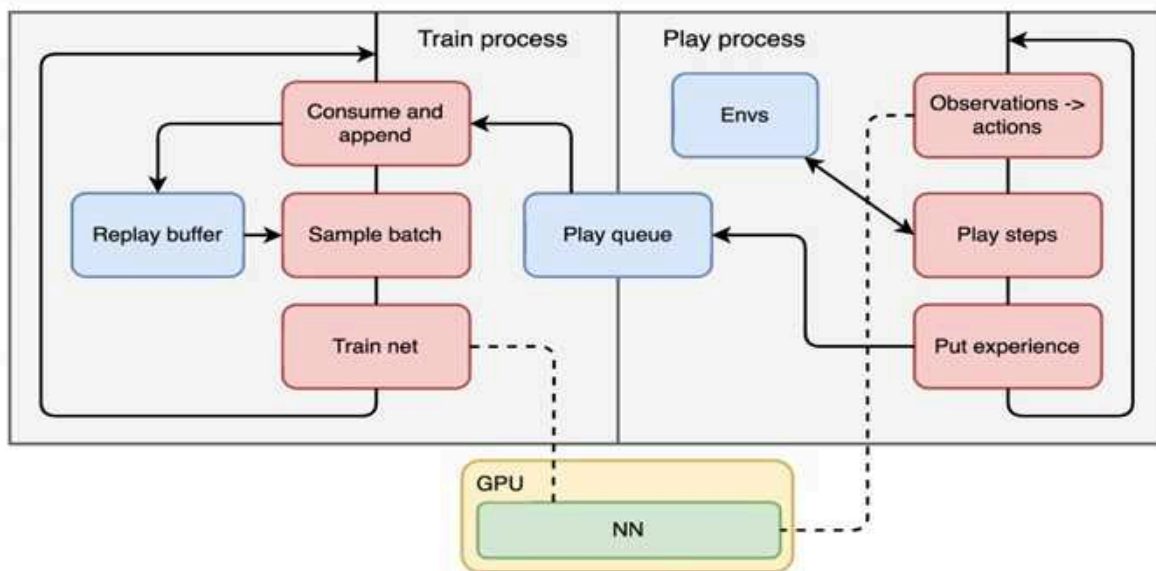
Figure 9.7: The parallel version of the training and play steps
