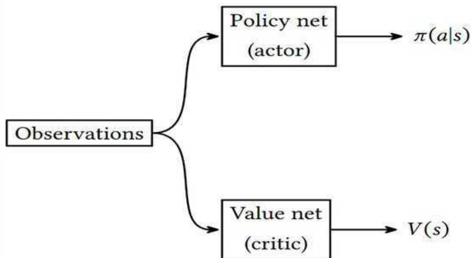
Figure 12.4: The A2C architecture
