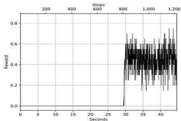
Figure 5.10: The reward dynamics on FrozenLake-8x8
