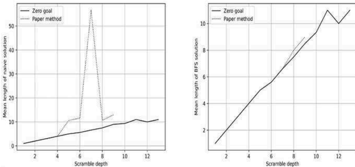
Figure 21.12: A comparison of naive (left) and BFS (right) solution lengths for 3 \times 3 cube
