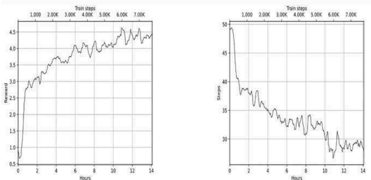
Figure 13.11: Training reward (left) and episode steps (right) on 200 games
