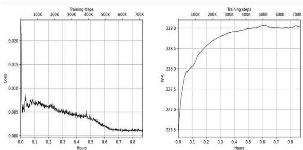
Figure 9.2: Loss and FPS during the training of baseline version
