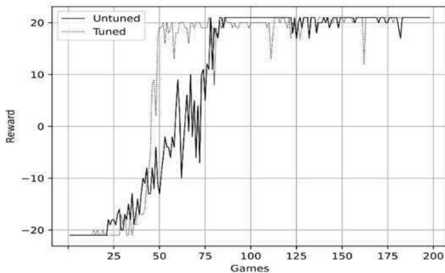
Figure 8.30: Raw reward for untuned and tuned combined DQN
