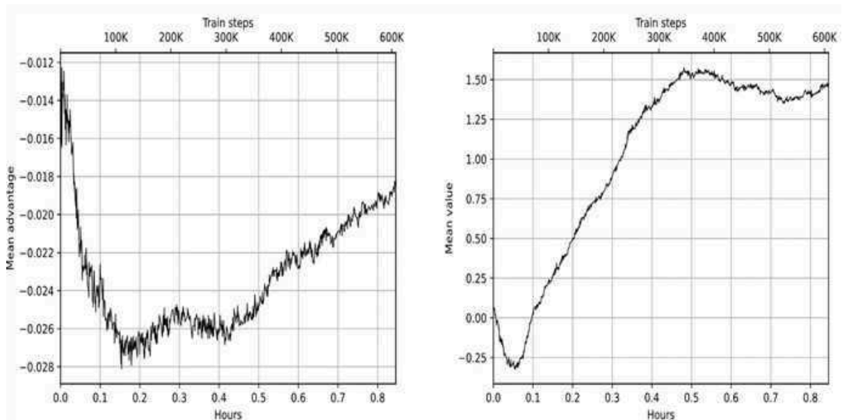
Figure 8.18: Mean advantage (left) and value (right) on a fixed set of states
