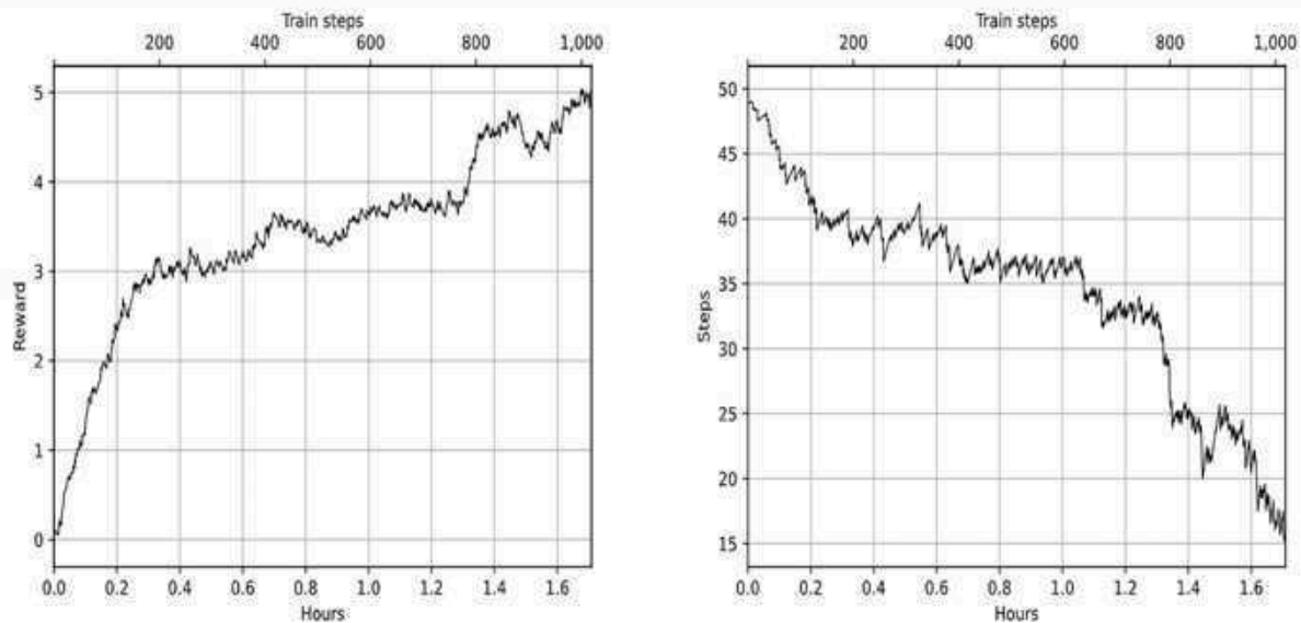
Figure 13.8: Training reward (left) and count of steps in episodes (right) for training on 20 games
