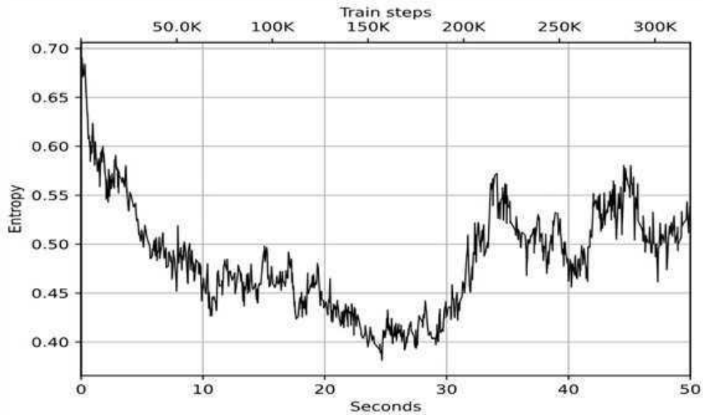
Figure 11.6: Entropy during the training
