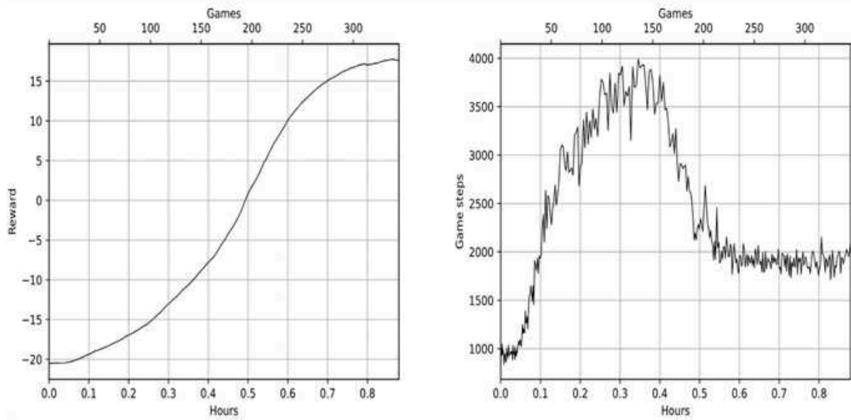
Figure 9.1: Reward and episode length in baseline version
