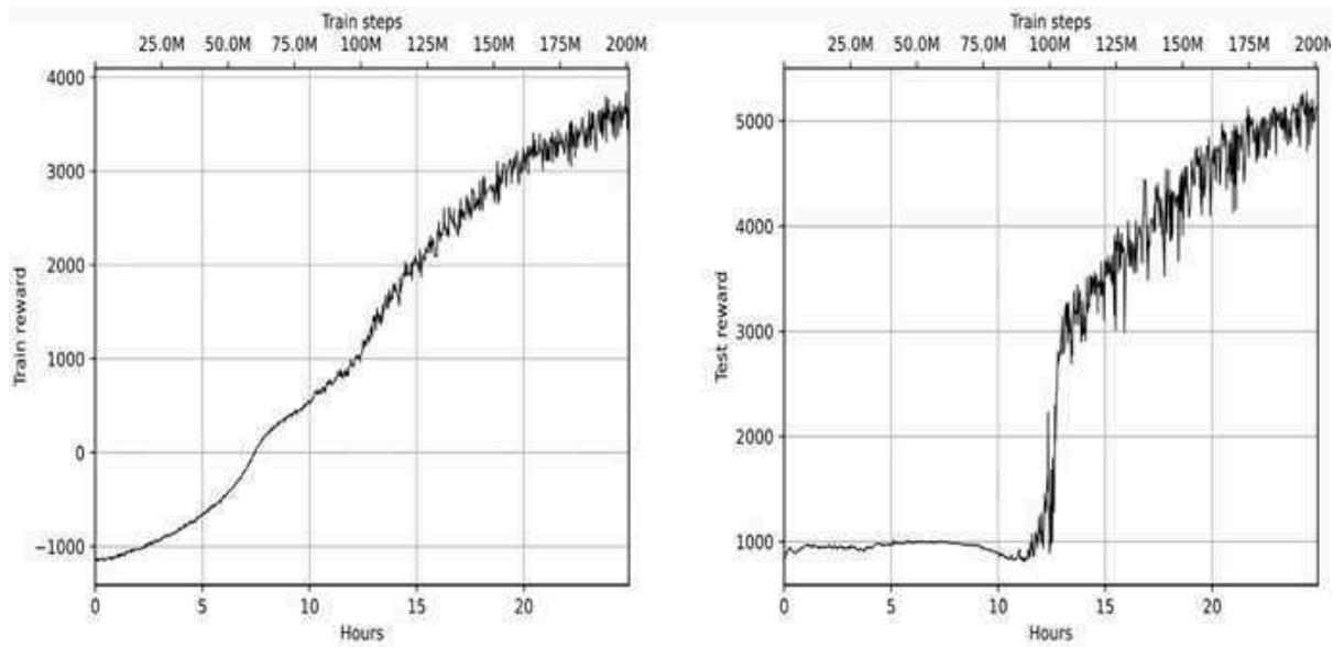
Figure 16.5: The reward during training (left) and the test reward (right) for Ant on MuJoCo
