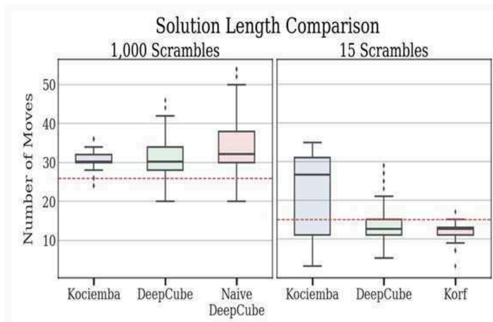
Figure 21.4: The length of solutions found by various solvers
