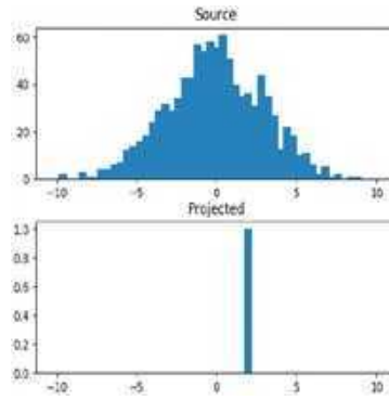
Figure 8.22: The projection of distribution for the final step in the episode
