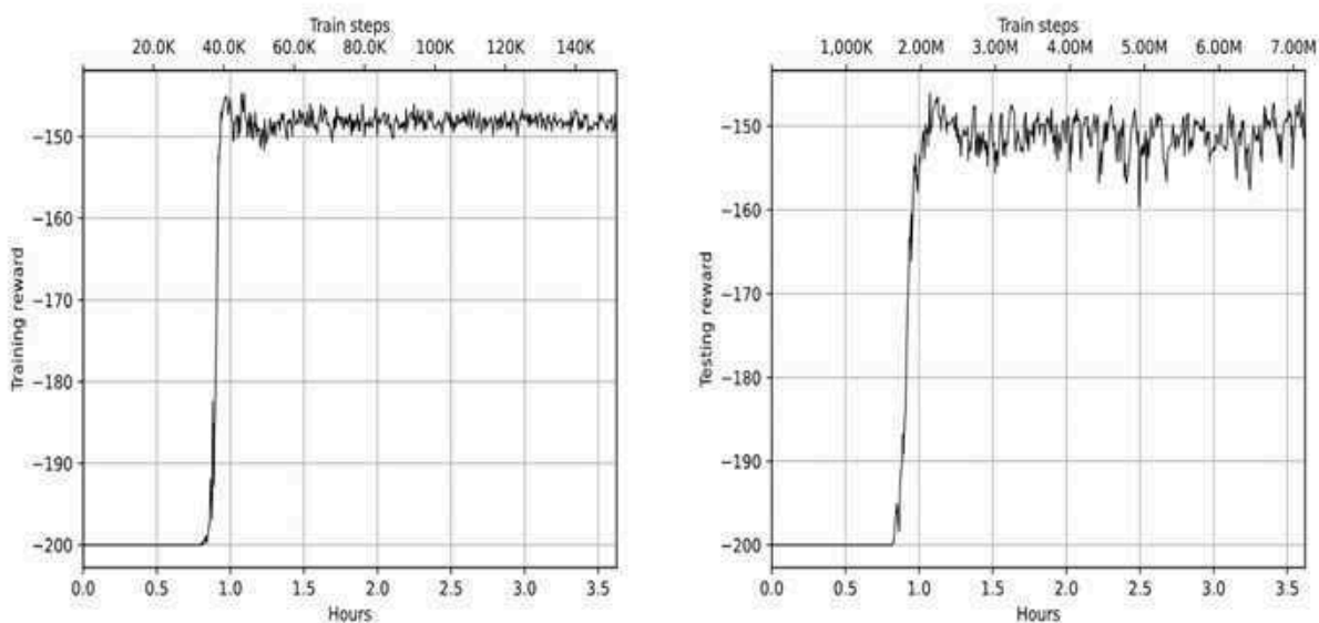
Figure 18.8: The training reward (left) and test rewards (right) on plain PPO
