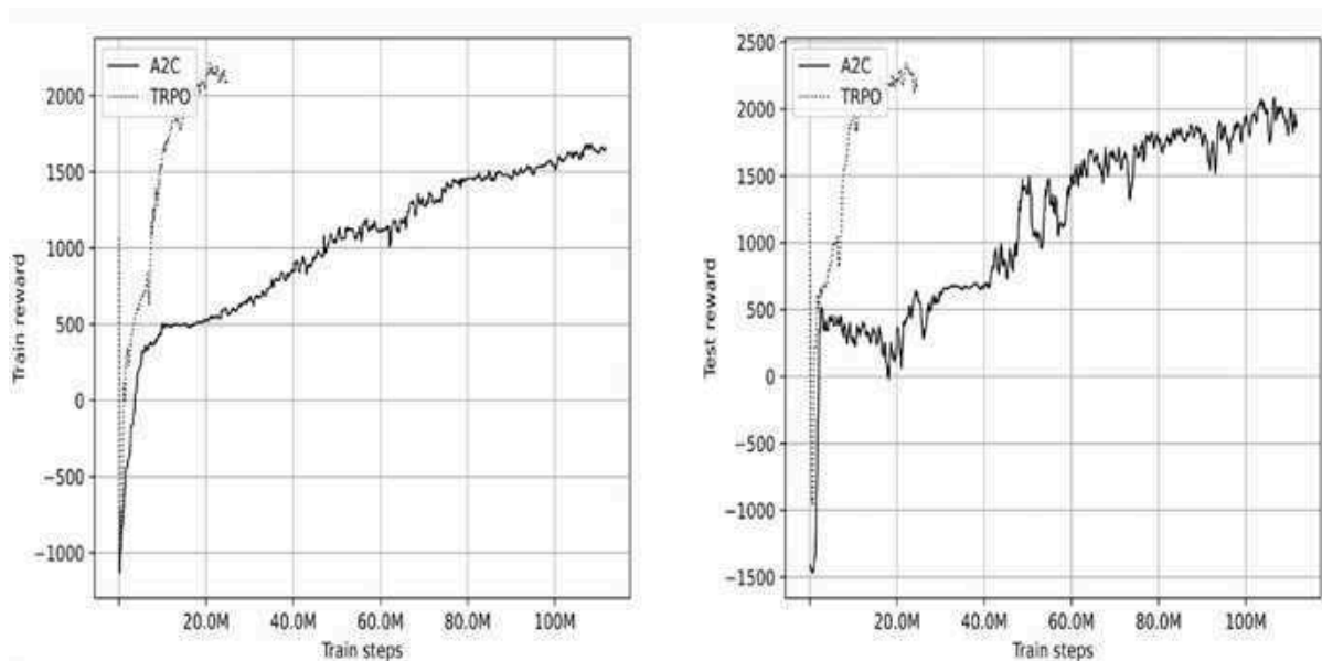
Figure 16.10: The reward during training (left) and test reward (right) for HalfCheetah on PyBullet
