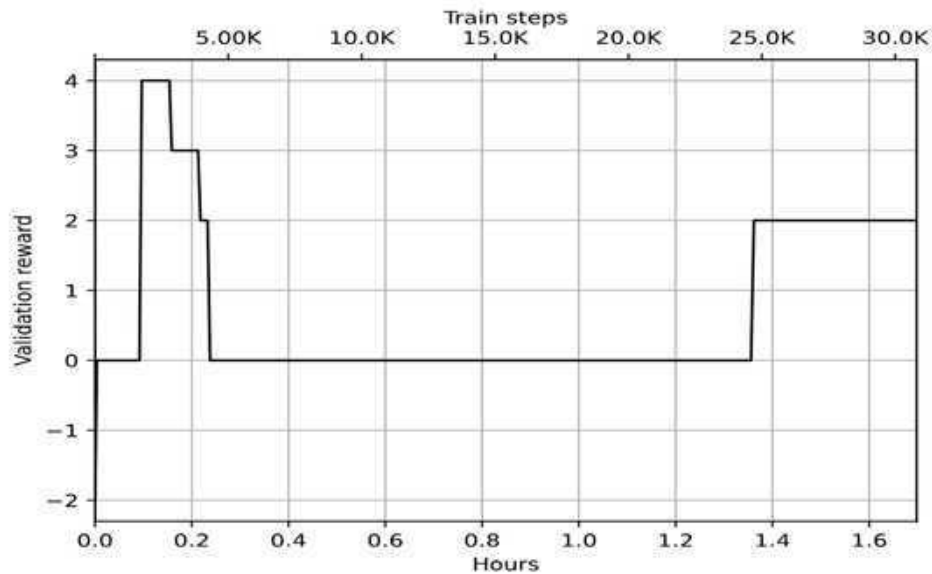
Figure 13.9: Validation reward during the training on 20 games
