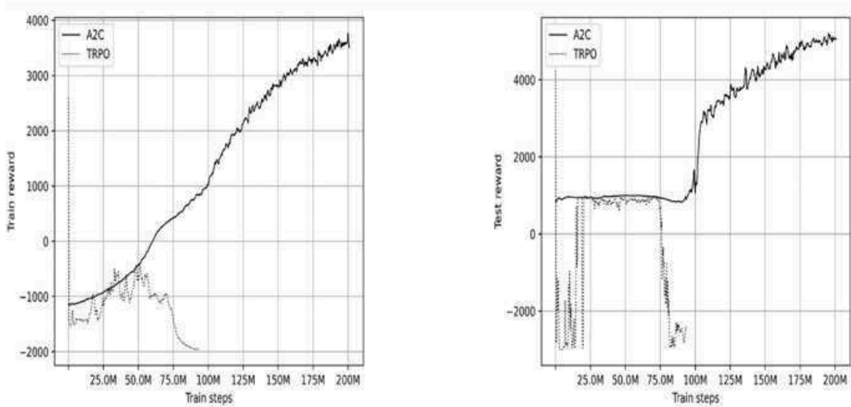
Figure 16.13: The reward during training (left) and the test reward (right) for Ant on MuJoCo
