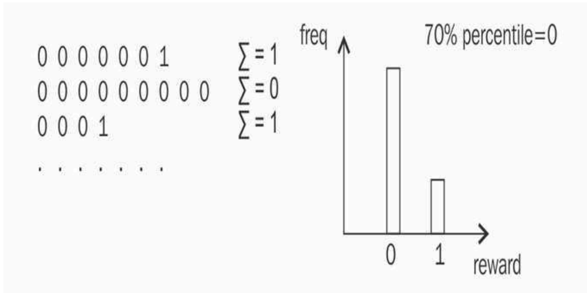
Figure 4.10: Reward distribution of the FrozenLake environment
