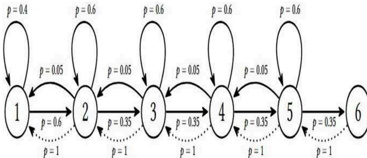
Figure 18.2: The full transition diagram for the River Swim environment
