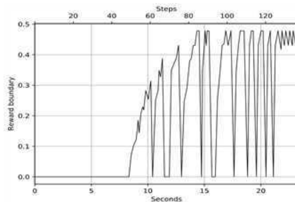
Figure 4.14: The reward boundary of the nonslippery version
