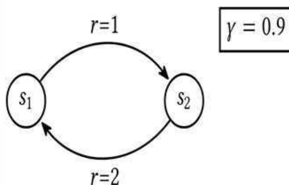
Figure 5.7: A sample environment with a loop in the transition diagram
