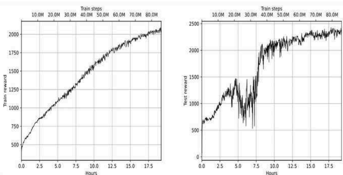
Figure 16.4: The reward during training (left) and the test reward (right) for Ant on PyBullet
