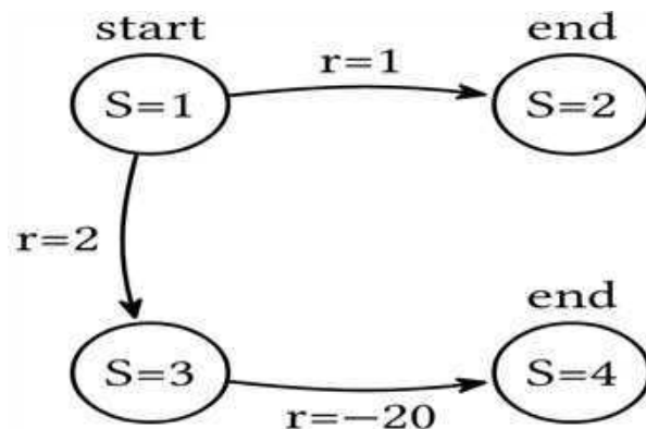
Figure 5.2: The same environment, with an extra state added
