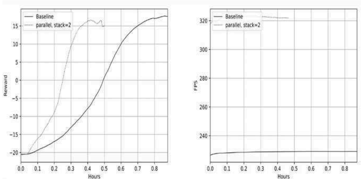
Figure 9.10: Reward and FPS in the baseline and “parallel and 2 frames” version
