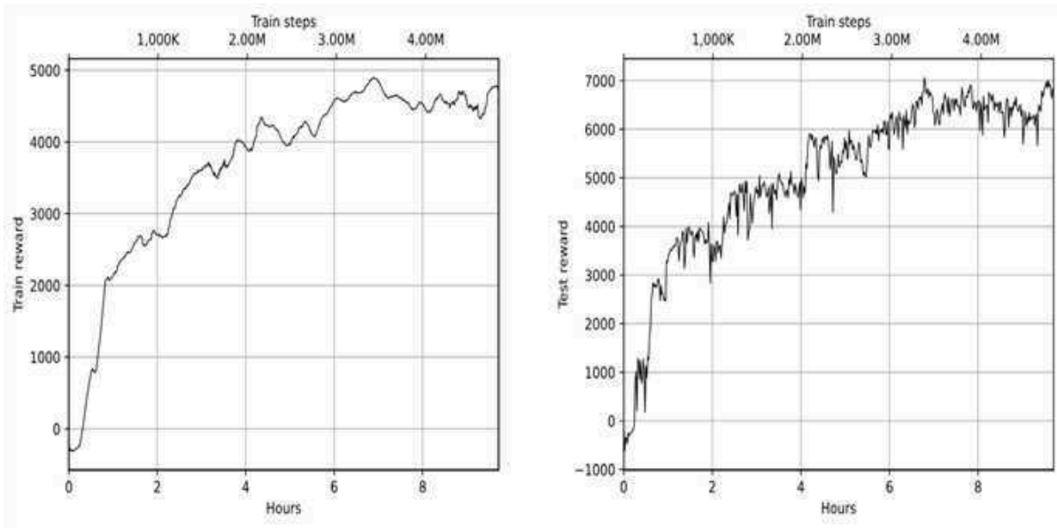
Figure 16.18: The reward during training (left) and the test reward (right) for HalfCheetah on MuJoCo
