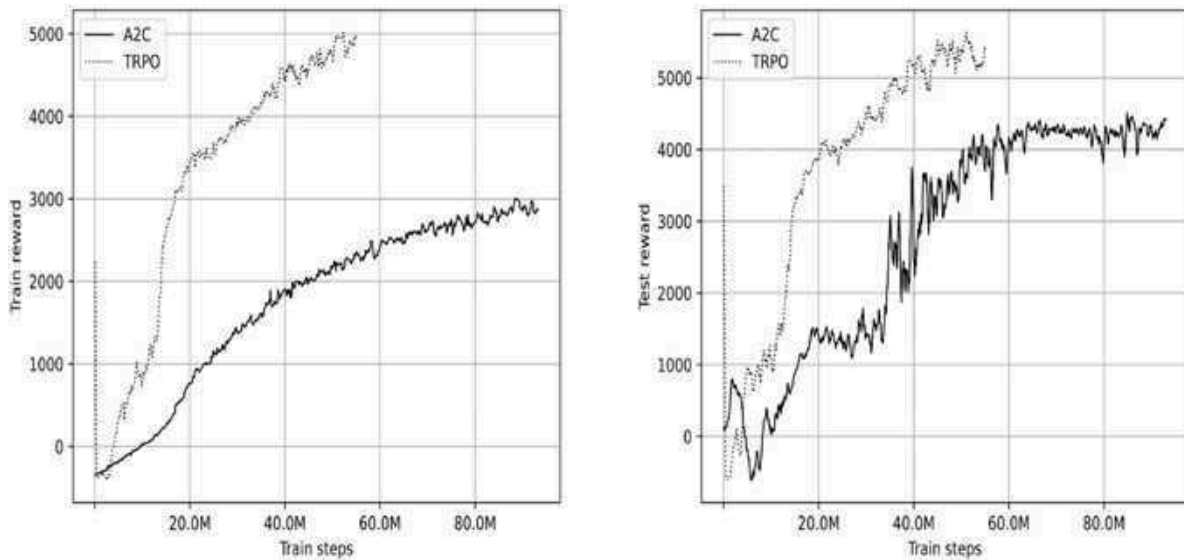
Figure 16.11: The reward during training (left) and the test reward (right) for HalfCheetah on MuJoCo
