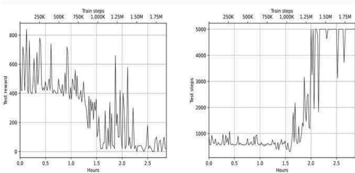
Figure 19.10: Test reward (left) and steps (right) during the fine-tuning
