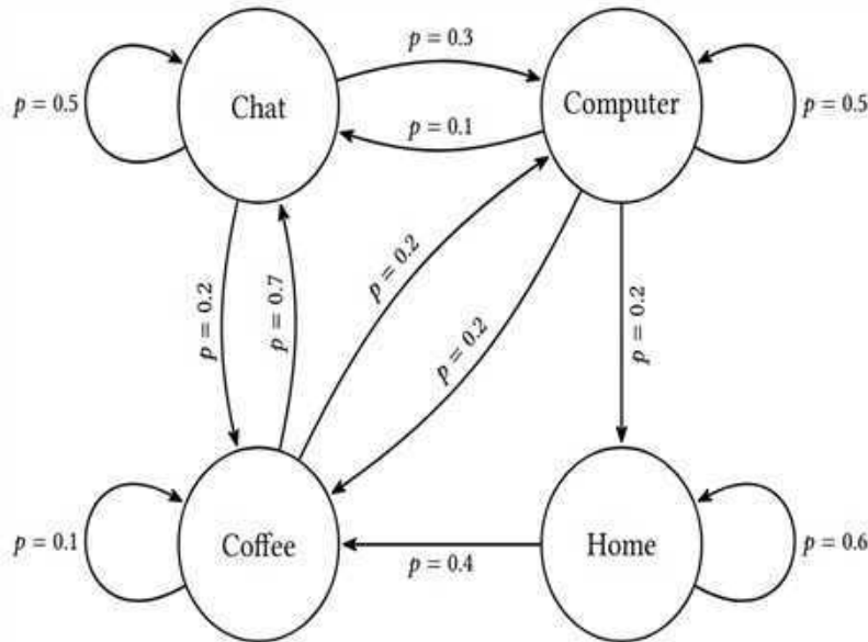
Figure 1.6: The state transition graph with transition probabilities
