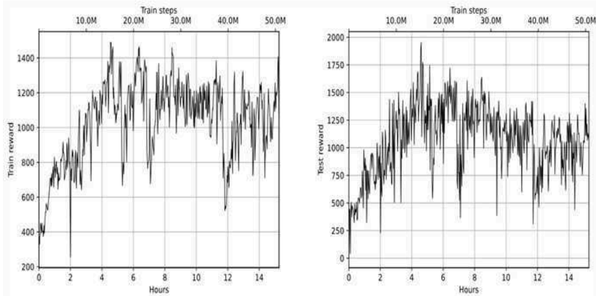
Figure 16.16: The reward during training (left) and the test reward (right) for Ant on PyBullet
