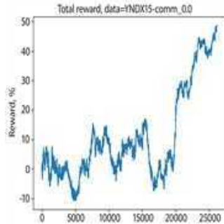
Figure 10.9: Trading profit on validation data without broker's commission
