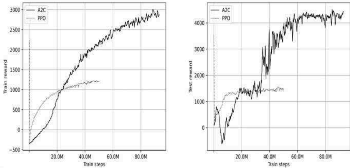
Figure 16.7: The reward during training (left) and the test reward (right) for HalfCheetah on MuJoCo
