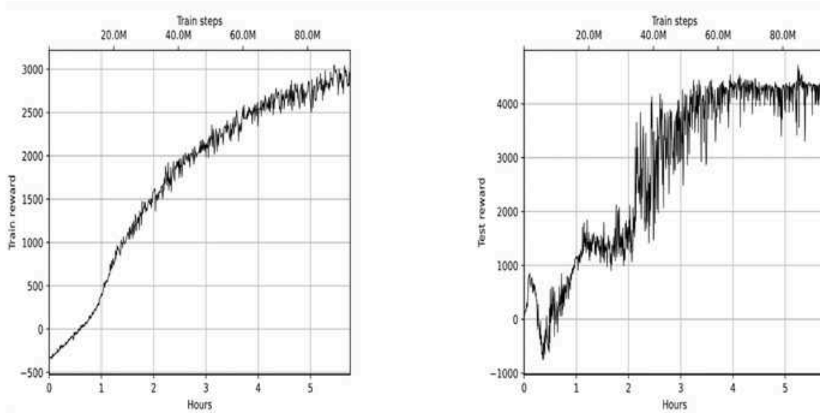
Figure 16.3: The reward during training (left) and the test reward (right) for HalfCheetah on MuJoCo
