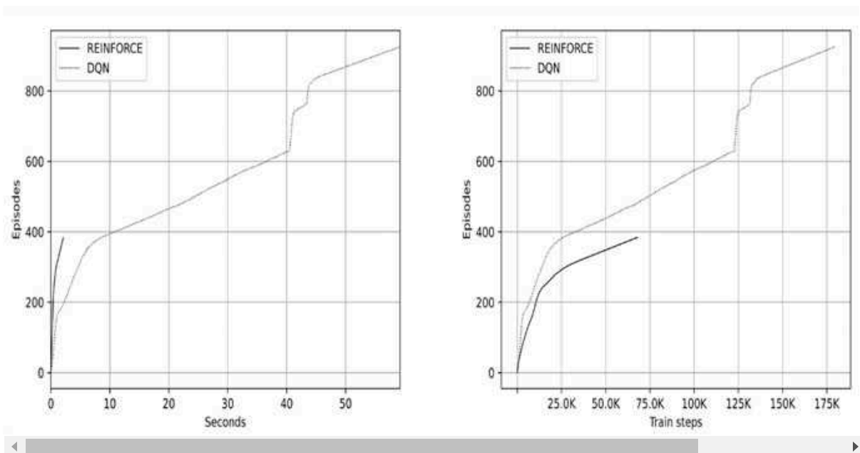
Figure 11.2: Count of episodes played over time (left) and training steps (right)
