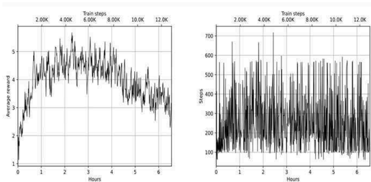
Figure 18.14: The average training reward (left) and count of steps (right) on DQN with noisy networks
