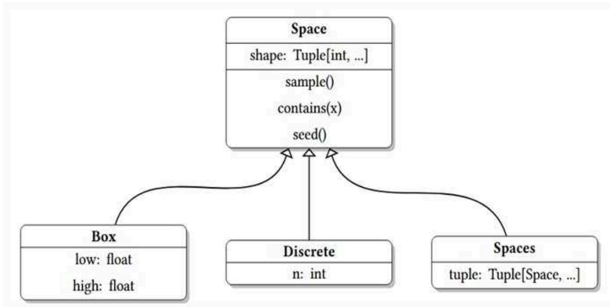
Figure 2.1: The hierarchy of the Space class in Gym
