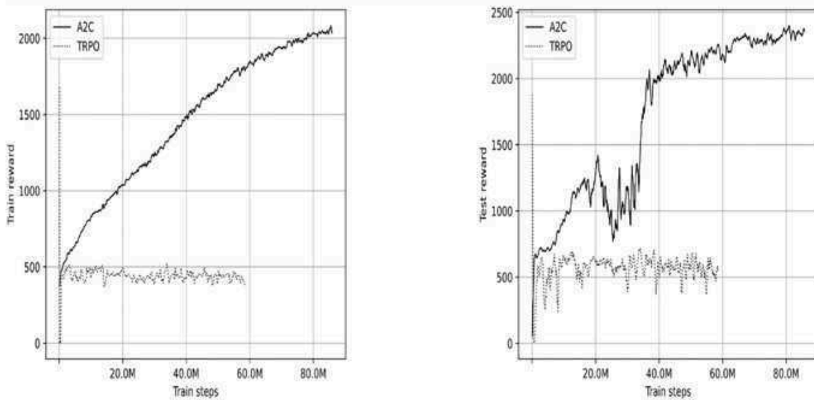
Figure 16.12: The reward during training (left) and the test reward (right) for Ant on PyBullet
