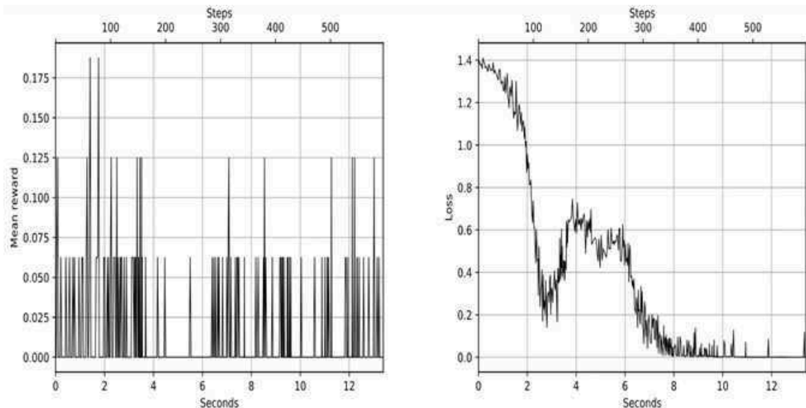
Figure 4.7: Mean reward (left) and loss (right) on the FrozenLake environment
