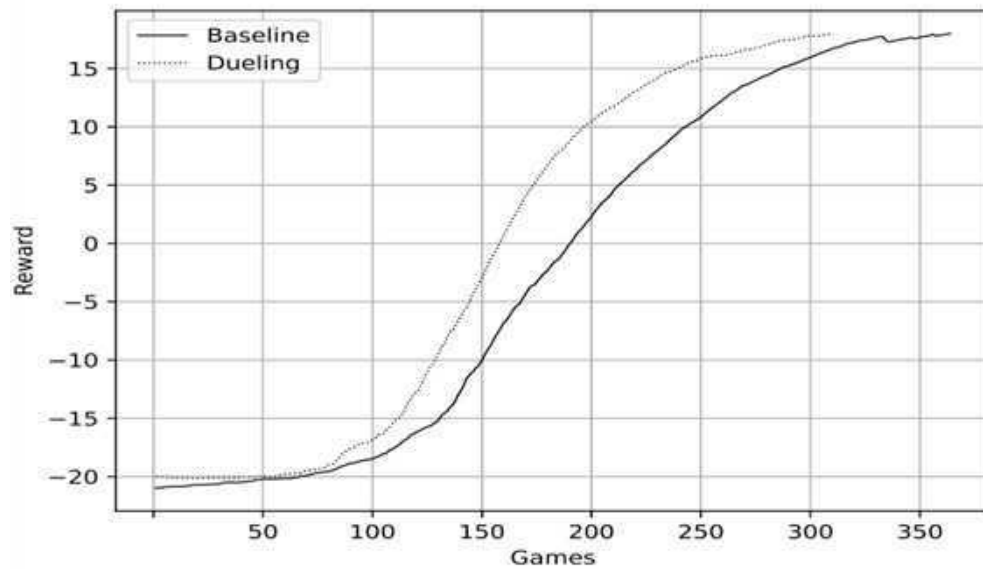
Figure 8.17: The reward dynamic of dueling DQN compared to the baseline version
