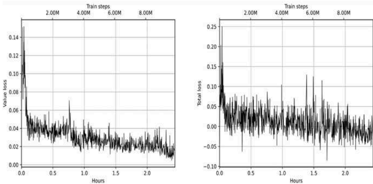
Figure 12.8: Value loss (left) and total loss (right)
