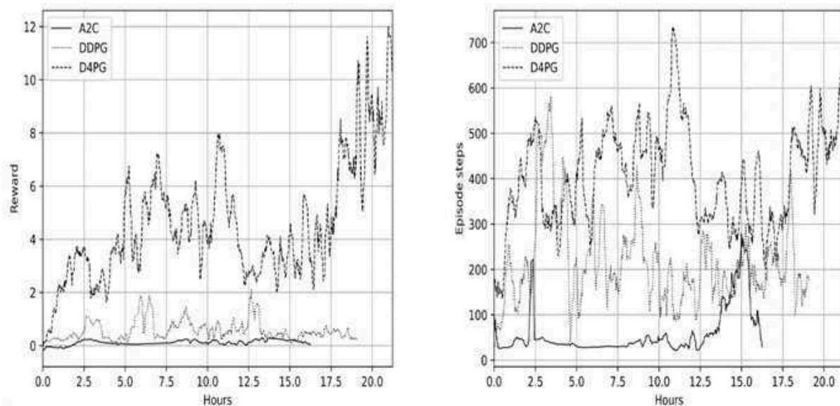
Figure 15.12: The reward (left) and steps (right) for test episodes
