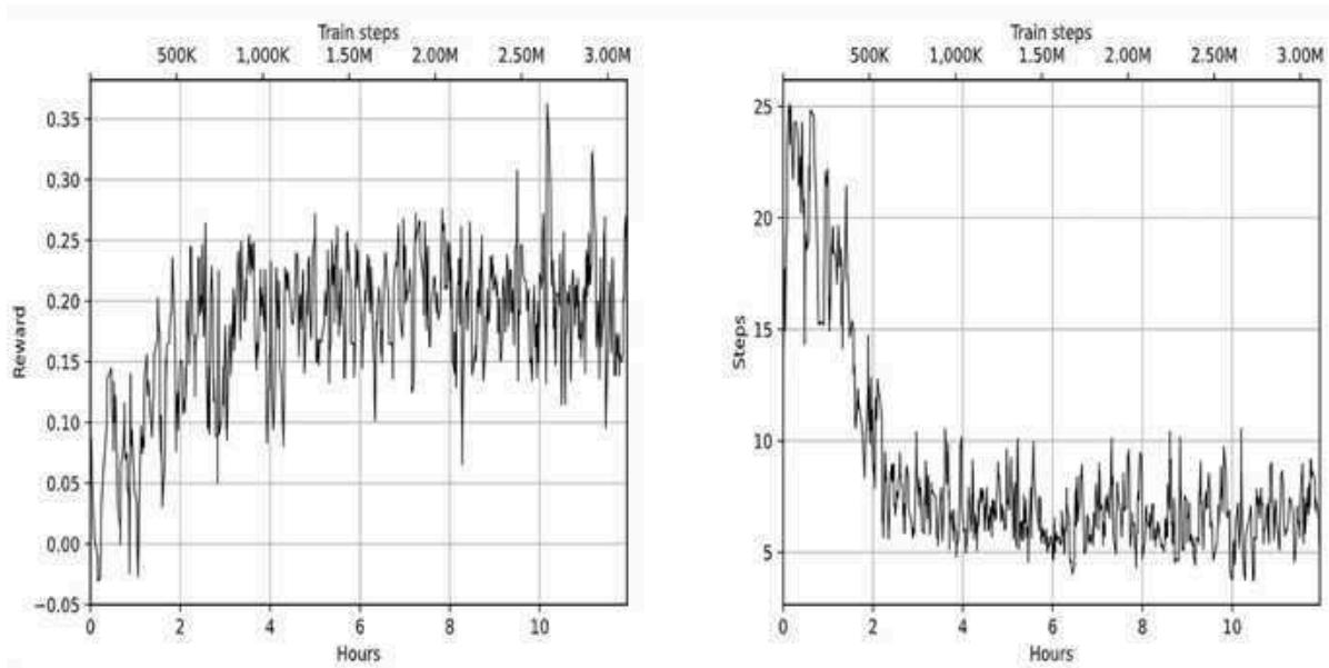
Figure 14.9: Training reward (left) and count of steps in episodes (right) on click-button
