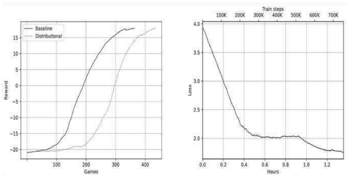
Figure 8.23: Reward dynamics (left) and loss decrease (right)
