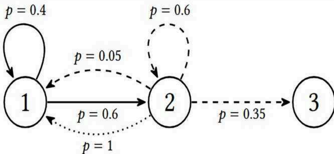
Figure 18.1: Transitions for the first two states of the River Swim environment
