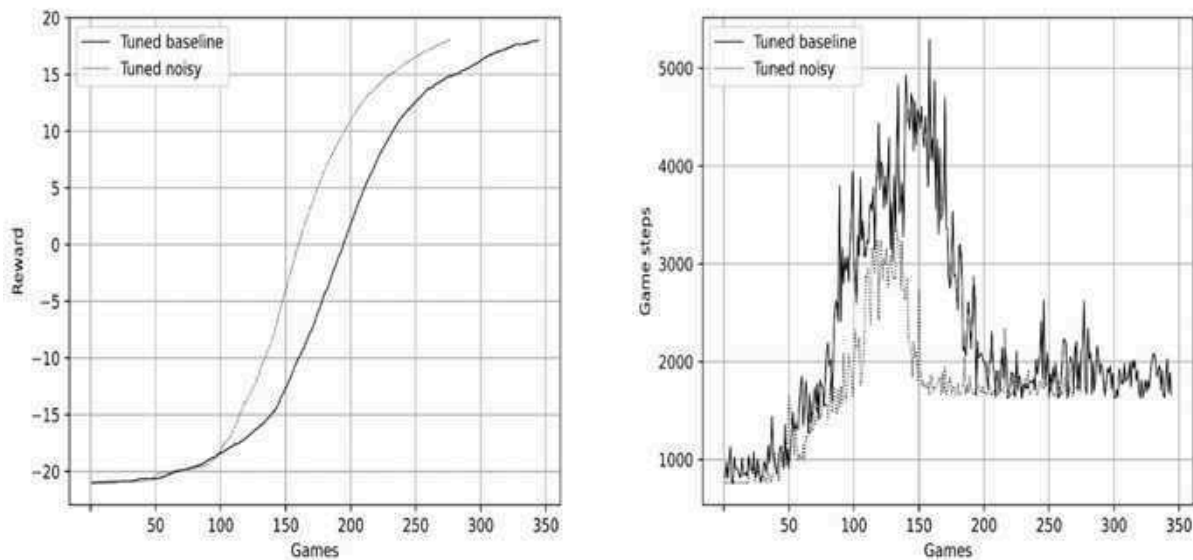
Figure 8.12: Comparison of tuned baseline DQN and tuned noisy network
