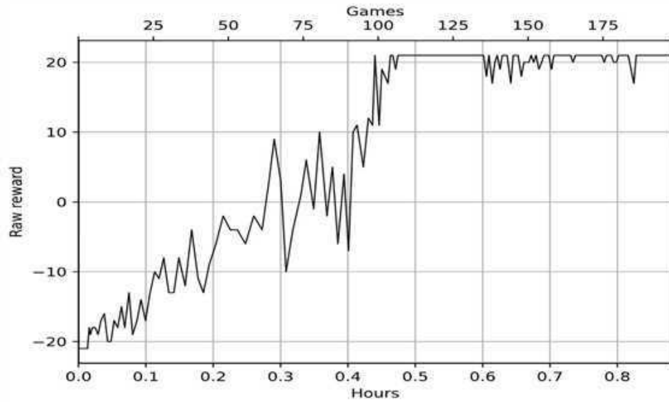
Figure 8.27: Raw reward for combined system
