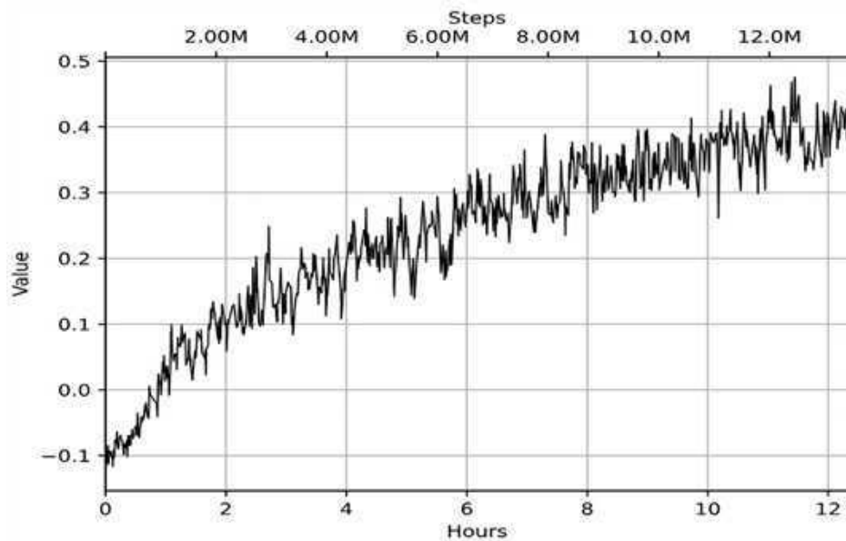
Figure 10.6: Value predicted for a random set of states
