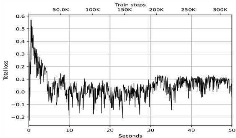
Figure 11.8: Total loss
