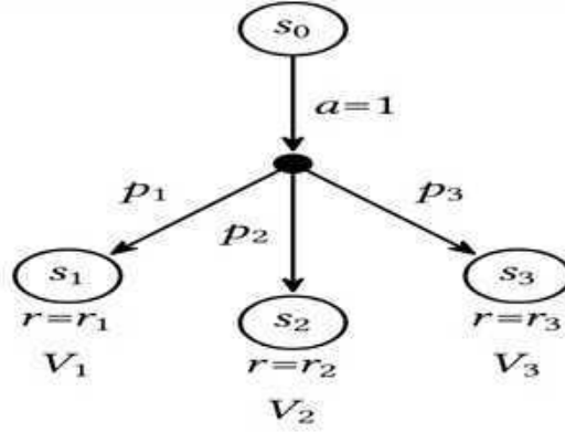
Figure 5.4: An example of the transition from the state in a stochastic case
