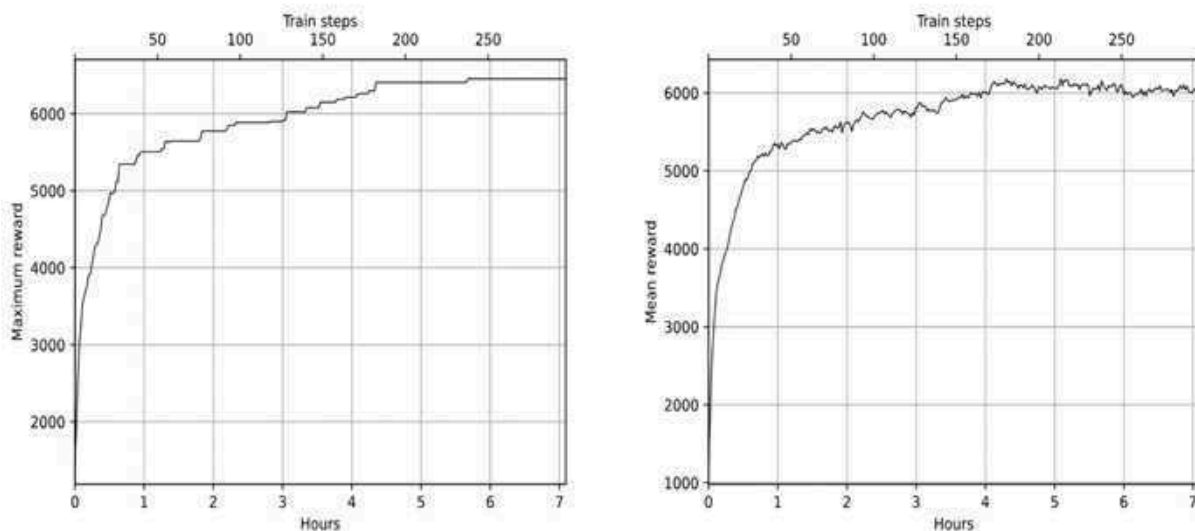
Figure 17.5: The maximum (left) and mean rewards (right) for GA on HalfCheetah
