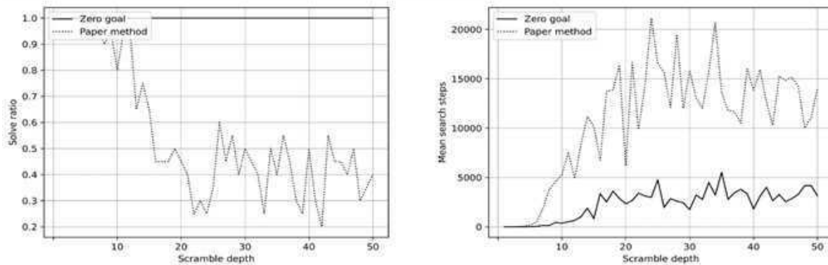
Figure 21.9: The ratio of solved 2 \times 2 cubes (left) and average count of MCTS searches needed for various scramble depths
