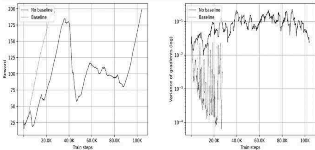
Figure 12.2: Smoothed reward (left) and variance (right)
