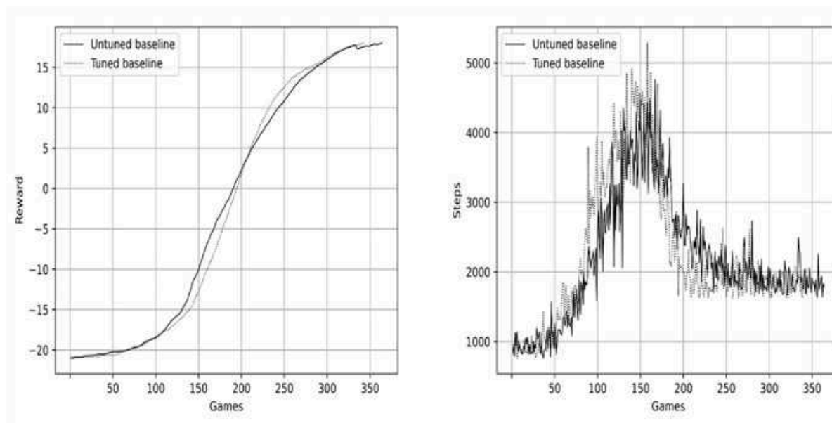
Figure 8.3: Plots with reward (left) and count of steps per episode (right) for tuned and untuned hyperparameters
