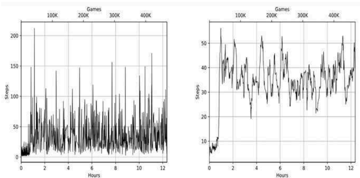
Figure 10.5: Length of the episodes. Raw values (left) and smoothed (right)
