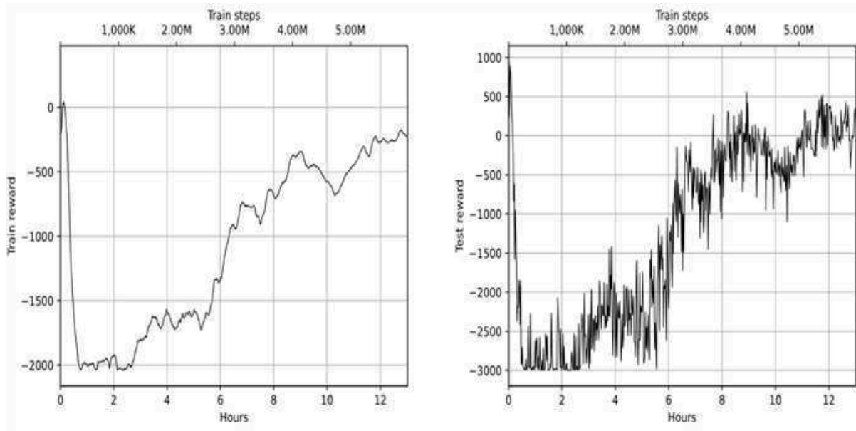
Figure 16.20: The reward during training (left) and the test reward (right) for Ant on MuJoCo
