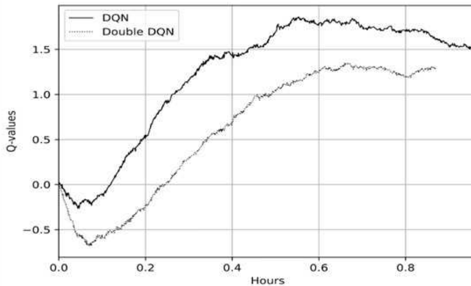
Figure 8.9: Values predicted by the network for held-out states
