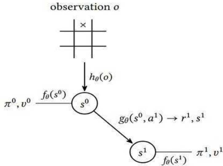
Figure 20.6: Monte-Carlo Tree Search in MuZero
