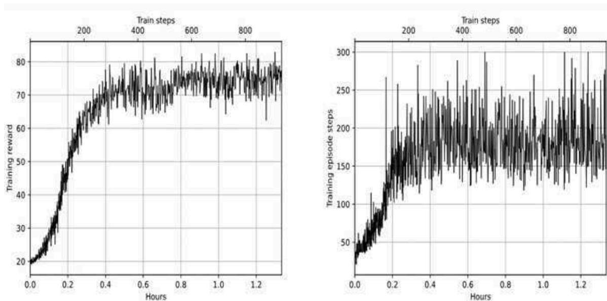
Figure 22.2: Average reward (left) and count of steps (right) from training episodes
