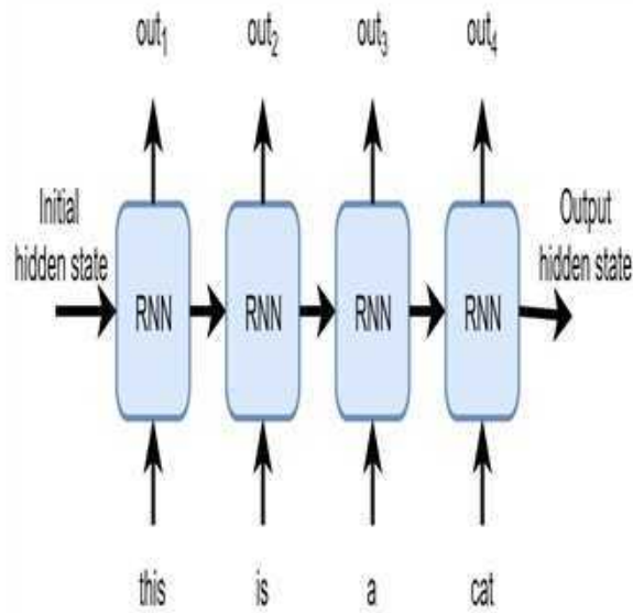
Figure 13.4: How an RNN is applied to a sentence
