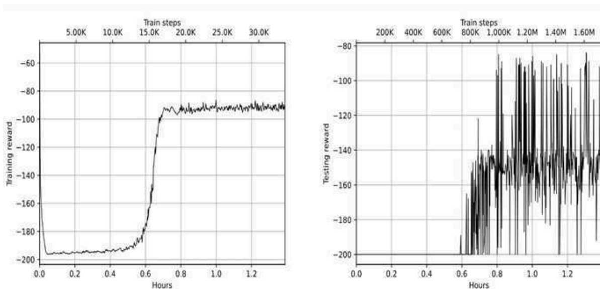
Figure 18.11: The training reward (left) and test rewards (right) on PPO with network distillation
