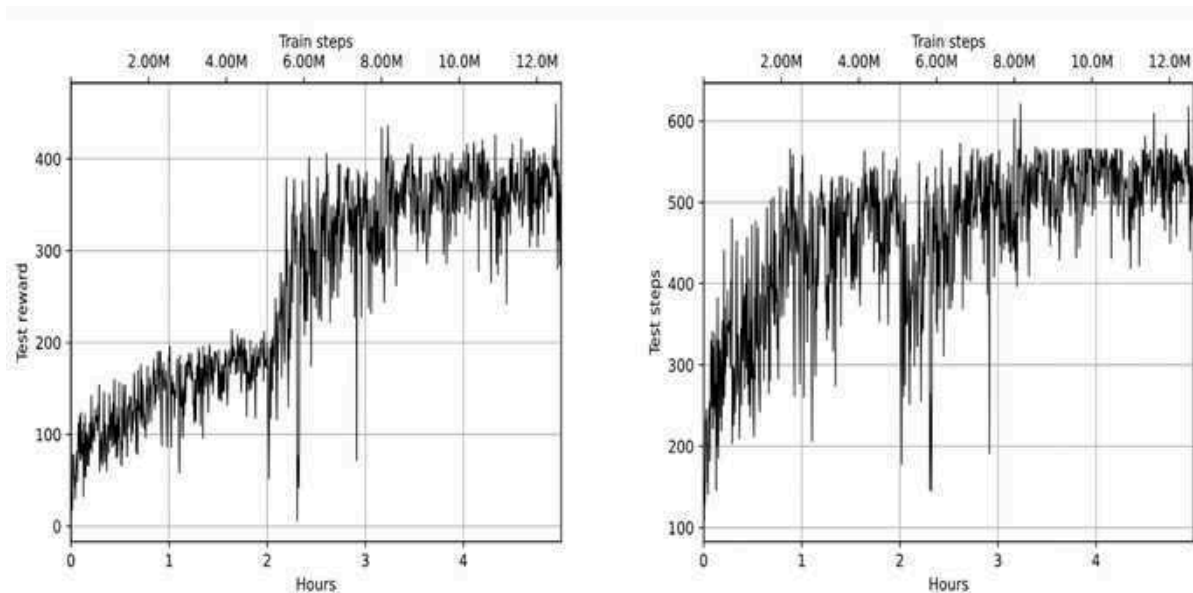
Figure 19.2: The reward (left) and steps (right) during the A2C training
