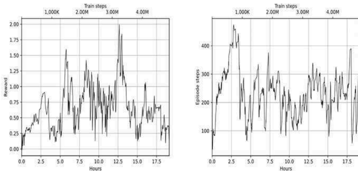
Figure 15.6: The reward (left) and steps (right) for training episodes
