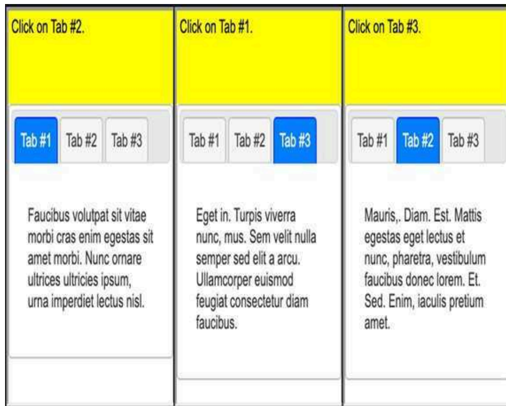
Figure 14.10: Tasks in the click-tab environment
