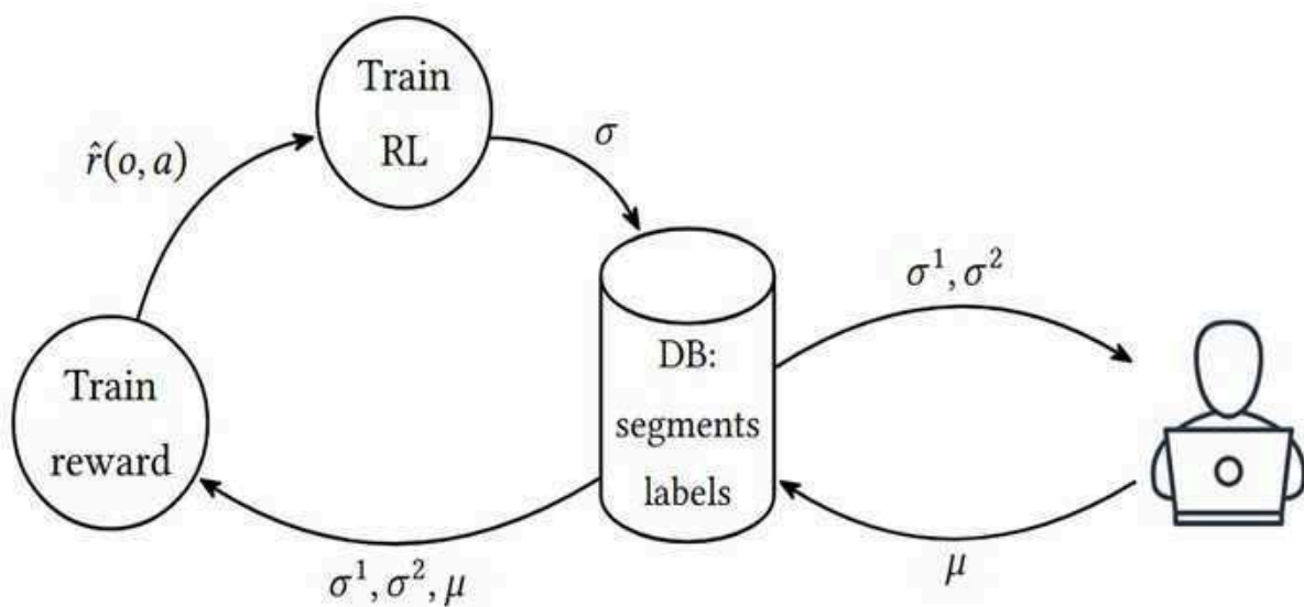
Figure 19.1: RLHF structure
