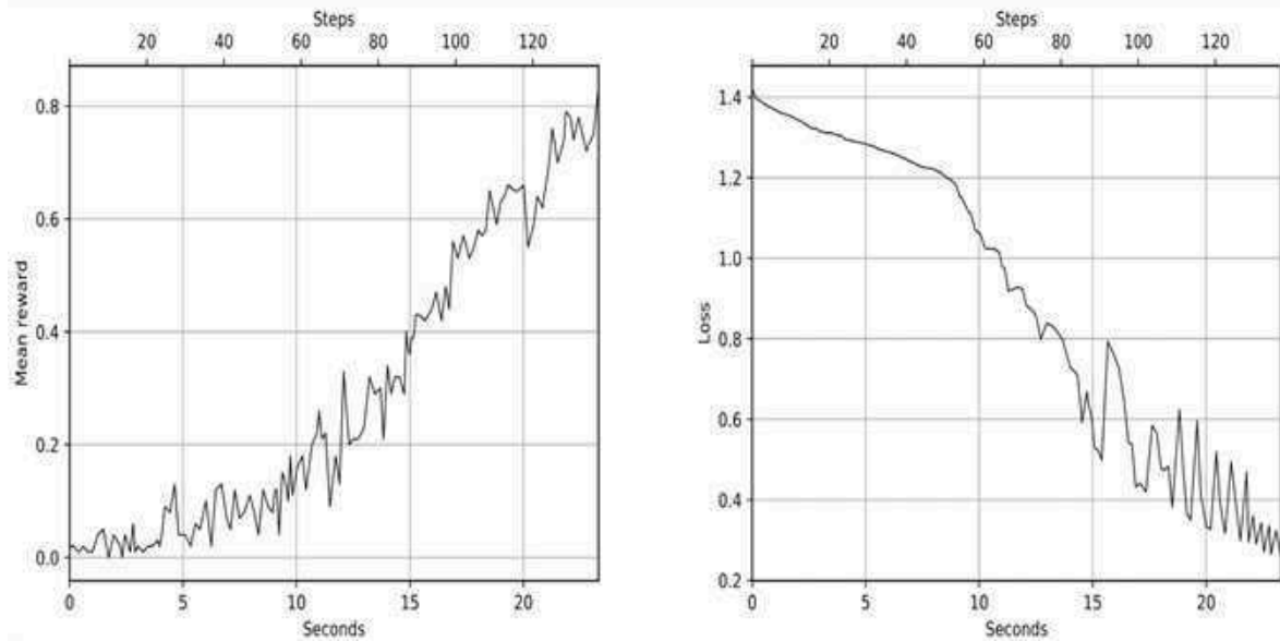
Figure 4.13: Mean reward (left) and loss (right) of the nonslippery version
