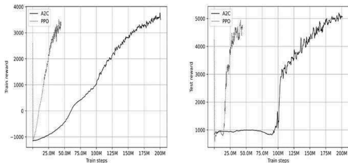
Figure 16.9: The reward during training (left) and the test reward (right) for Ant on MuJoCo
