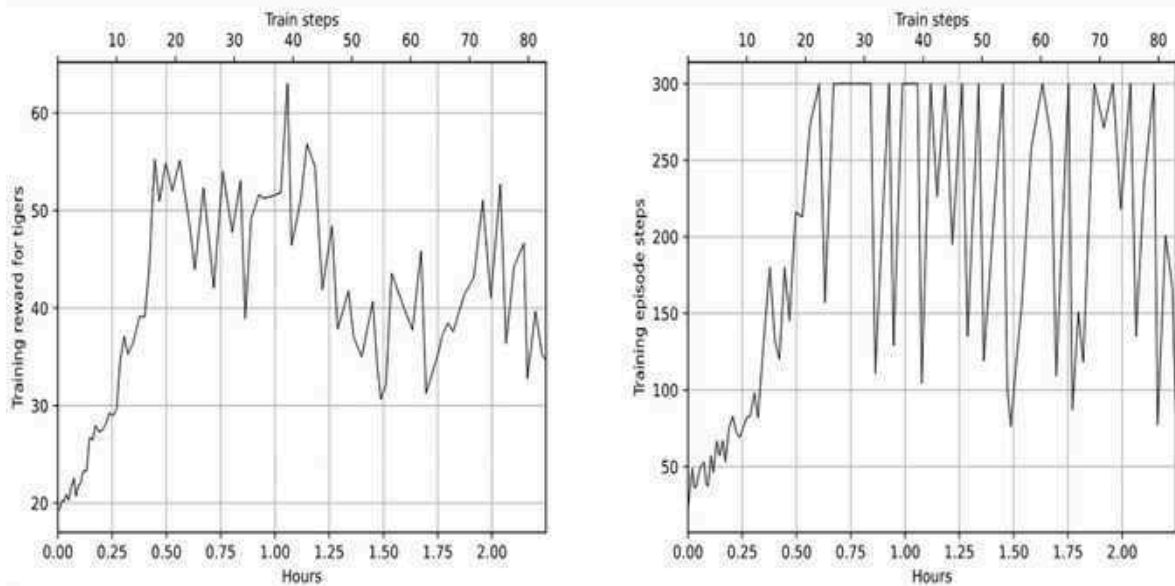
Figure 22.7: Average reward for tigers (left) and count of steps (right) from training episodes
