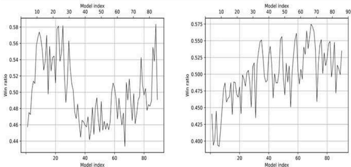
Figure 20.5: Win ratio for best models during the training, learning rate=0.1 (left) and learning rate=0.001 (right)
