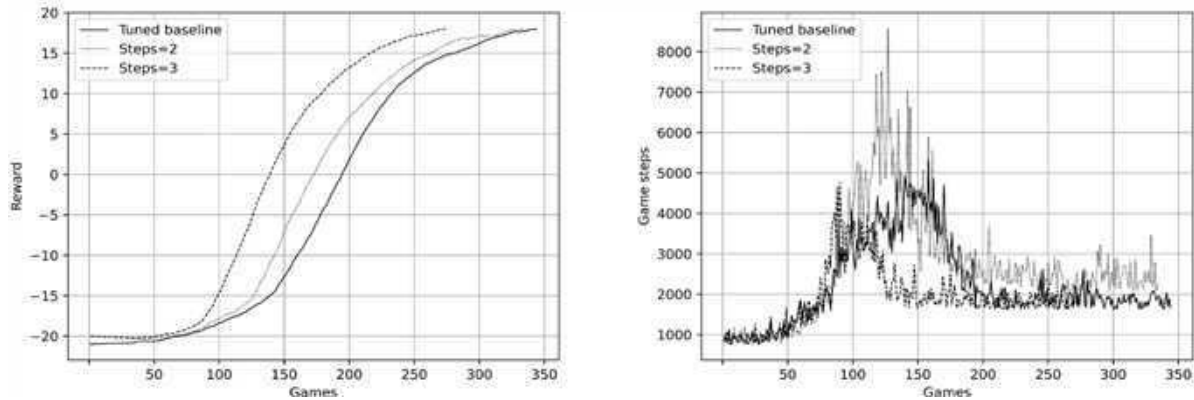
Figure 8.7: The reward and number of steps after hyperparameter tuning
