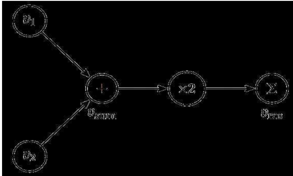
Figure 3.3: Graph representation of the expression
