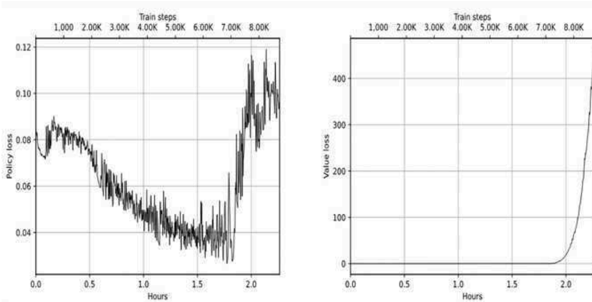
Figure 21.6: The policy loss (left) and value loss (right) during the typical run of the paper's method
