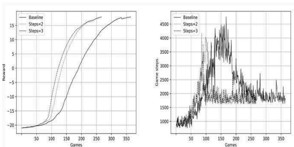
Figure 8.5: The reward and number of steps for basic (one-step) DQN and n -step versions
