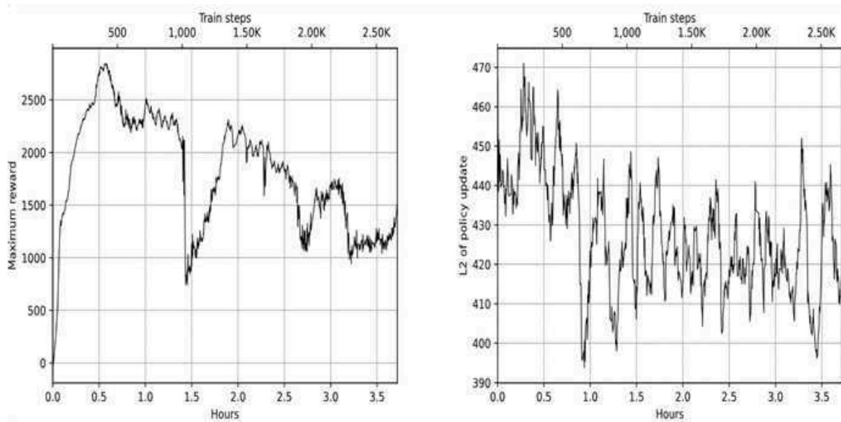
Figure 17.3: The maximum reward (left) and policy update (right) for ES on HalfCheetah
