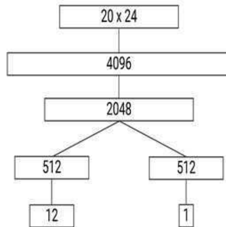
Figure 21.2: The NN architecture transforming the observation (top) to the action and value (bottom)
