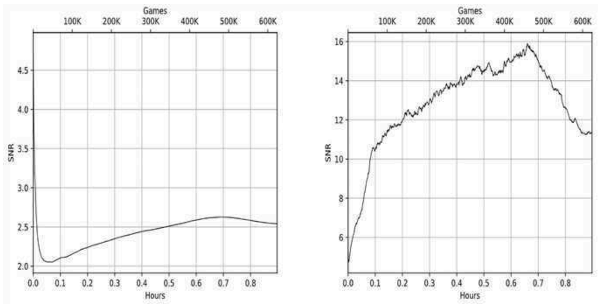
Figure 8.11: SNR change in layer 1 (left) and layer 2 (right)
