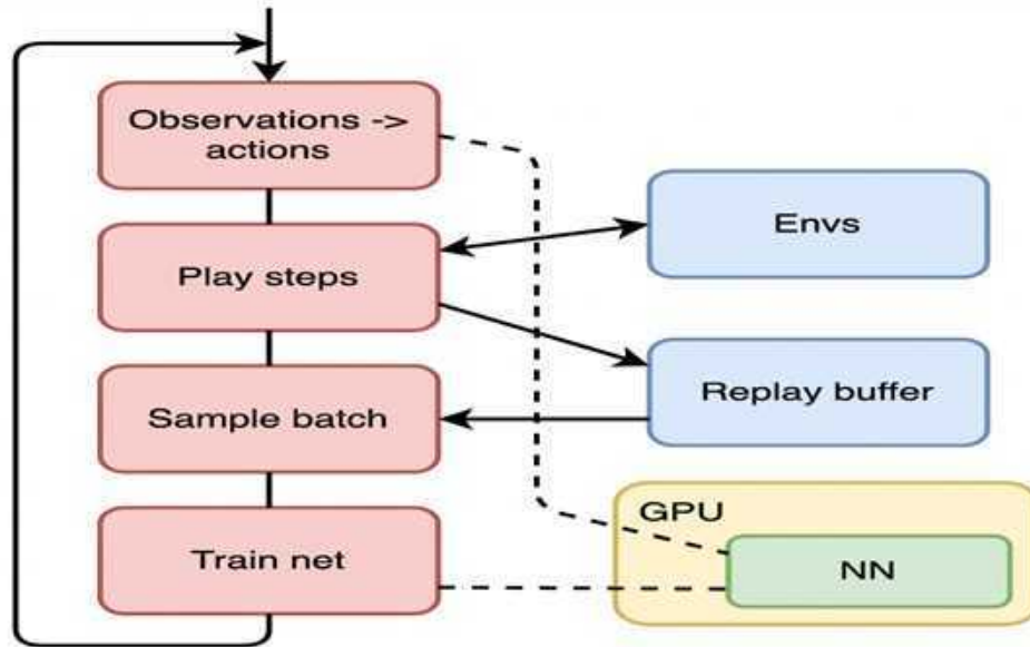
Figure 9.6: A sequential diagram of the training process
