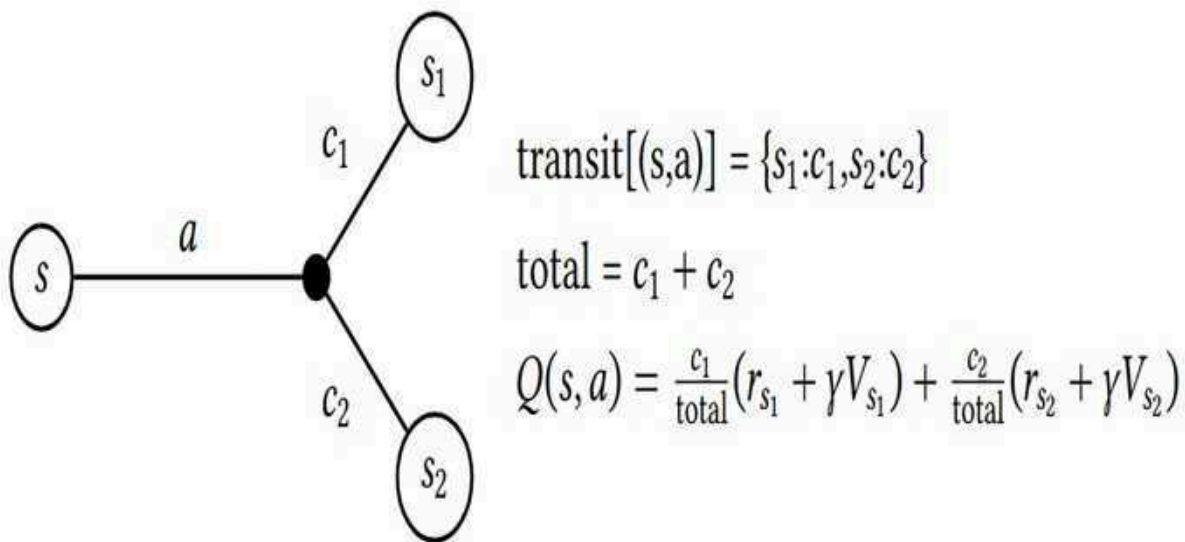
Figure 5.8: The calculation of the state's value
