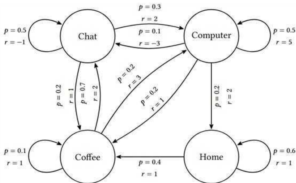
Figure 1.7: The state transition graph with transition probabilities and rewards
