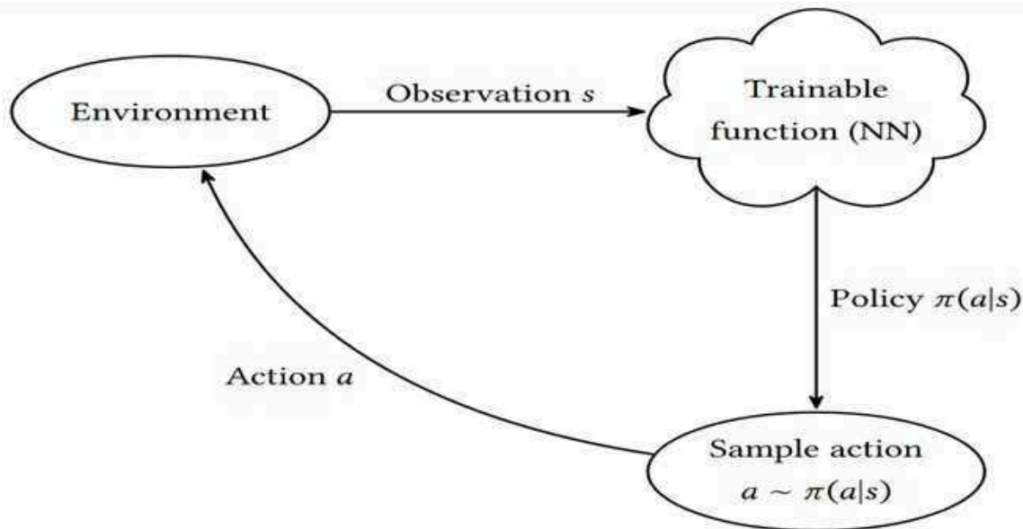
Figure 4.1: A high-level approach to policy-based RL
