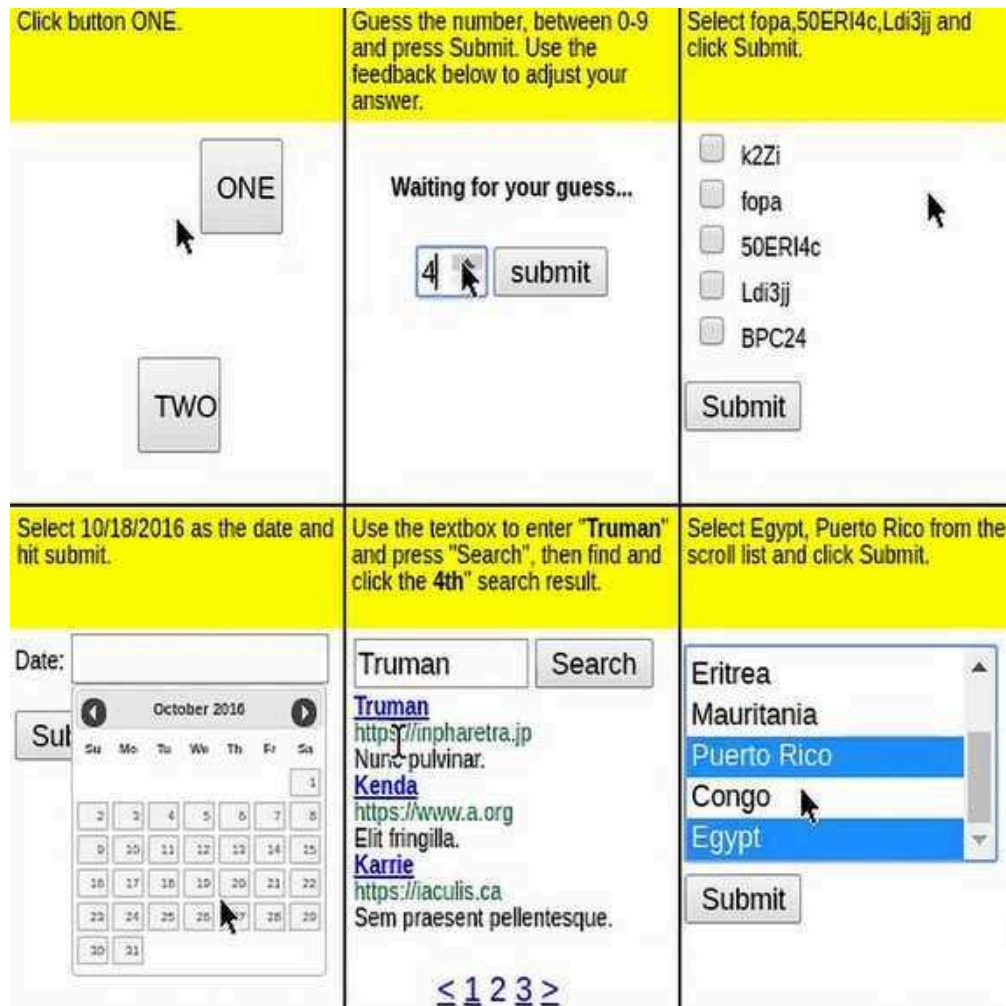
Figure 14.1: MiniWoB environments
