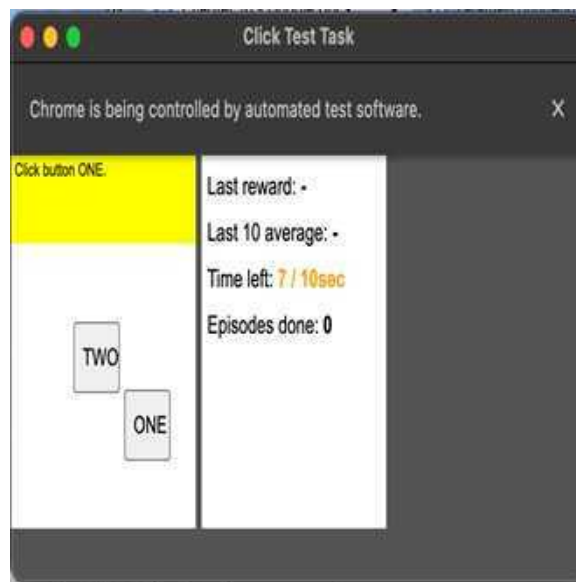
Figure 14.2: click-test-2 environment
