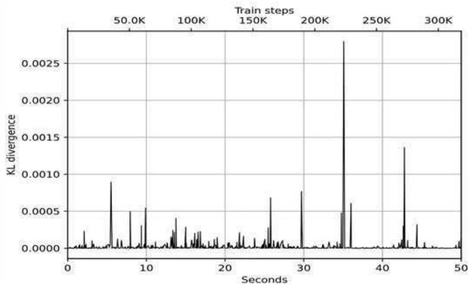
Figure 11.10: KL divergence
