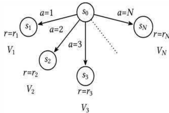
Figure 5.3: An abstract environment with N states reachable from the initial state
