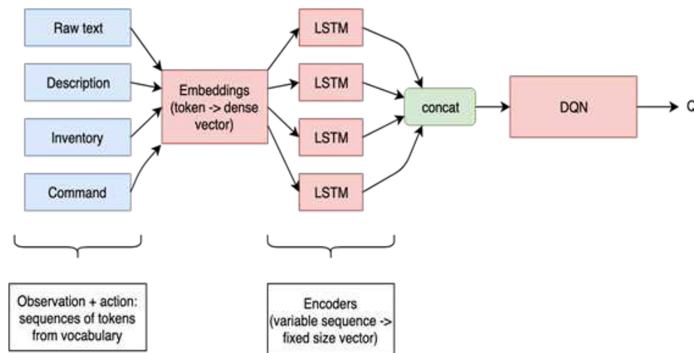
Figure 13.6: The architecture of the TextWorld baseline DQN
