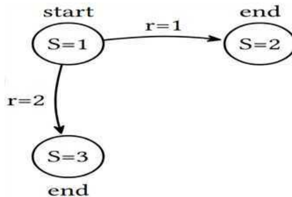
Figure 5.1: An example of an environment's state transition with rewards
