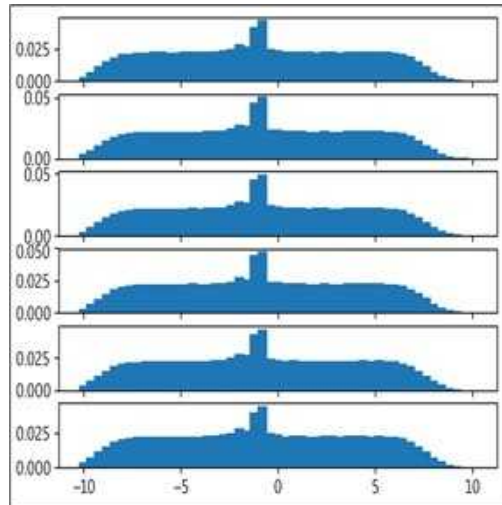
Figure 8.24: Probability distribution at the beginning of training
