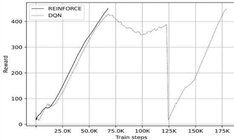
Figure 11.3: Reward dynamics for two methods
