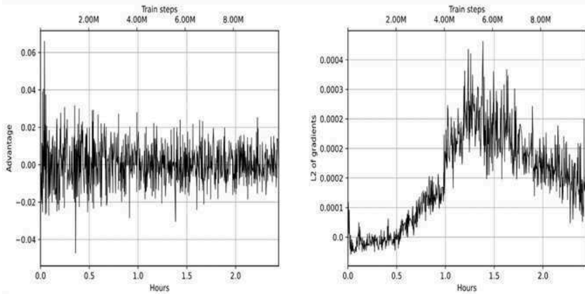
Figure 12.9: Advantage (left) and L2 of gradients (right)
