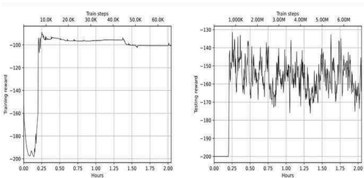
Figure 18.7: The training reward (left) and test rewards (right) on DQN with pseudo-count reward bonus
