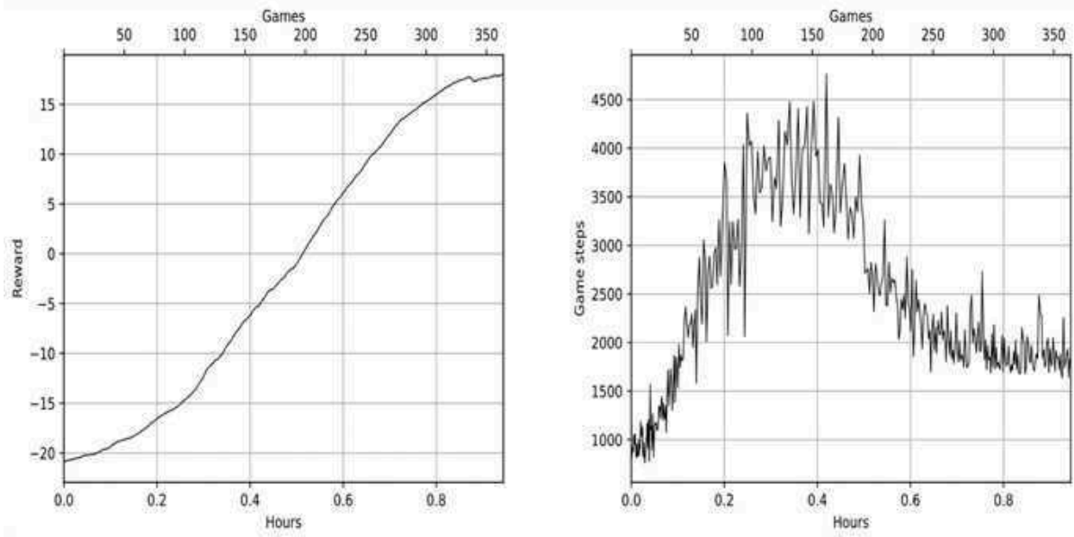
Figure 8.1: Plots with reward (left) and count of steps per episode (right)
