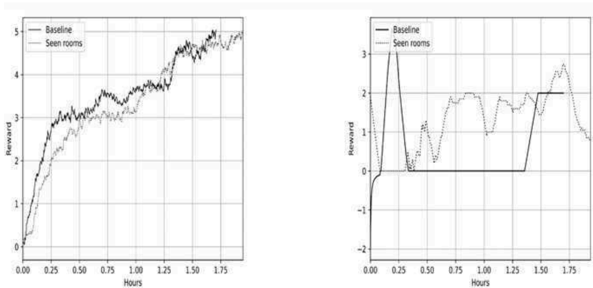
Figure 13.10: Training reward (left) and validation reward (right) on 20 games
