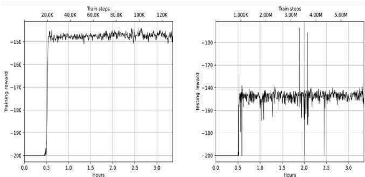
Figure 18.9: The training reward (left) and test rewards (right) on PPO with Noisy Networks
