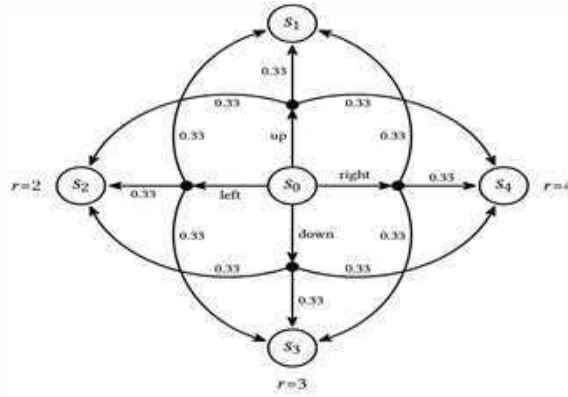
Figure 5.6: A transition diagram of the grid environment
