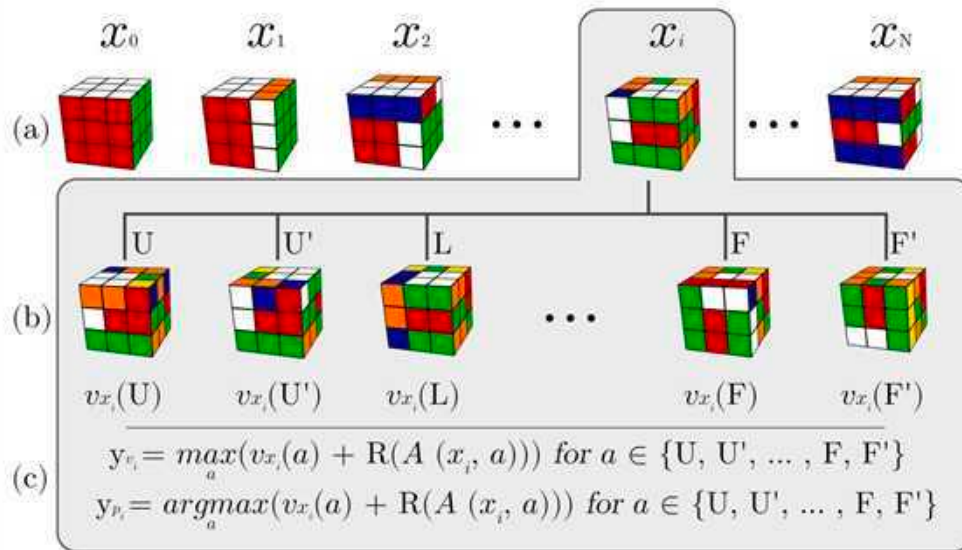
Figure 21.3: Data generation for training
